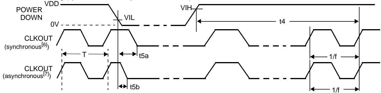
Power-up Timing
